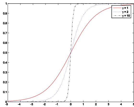
Figure 1: Transition Function with c=0 . Sensivity Analysis to the Slope Parameter \gamma
